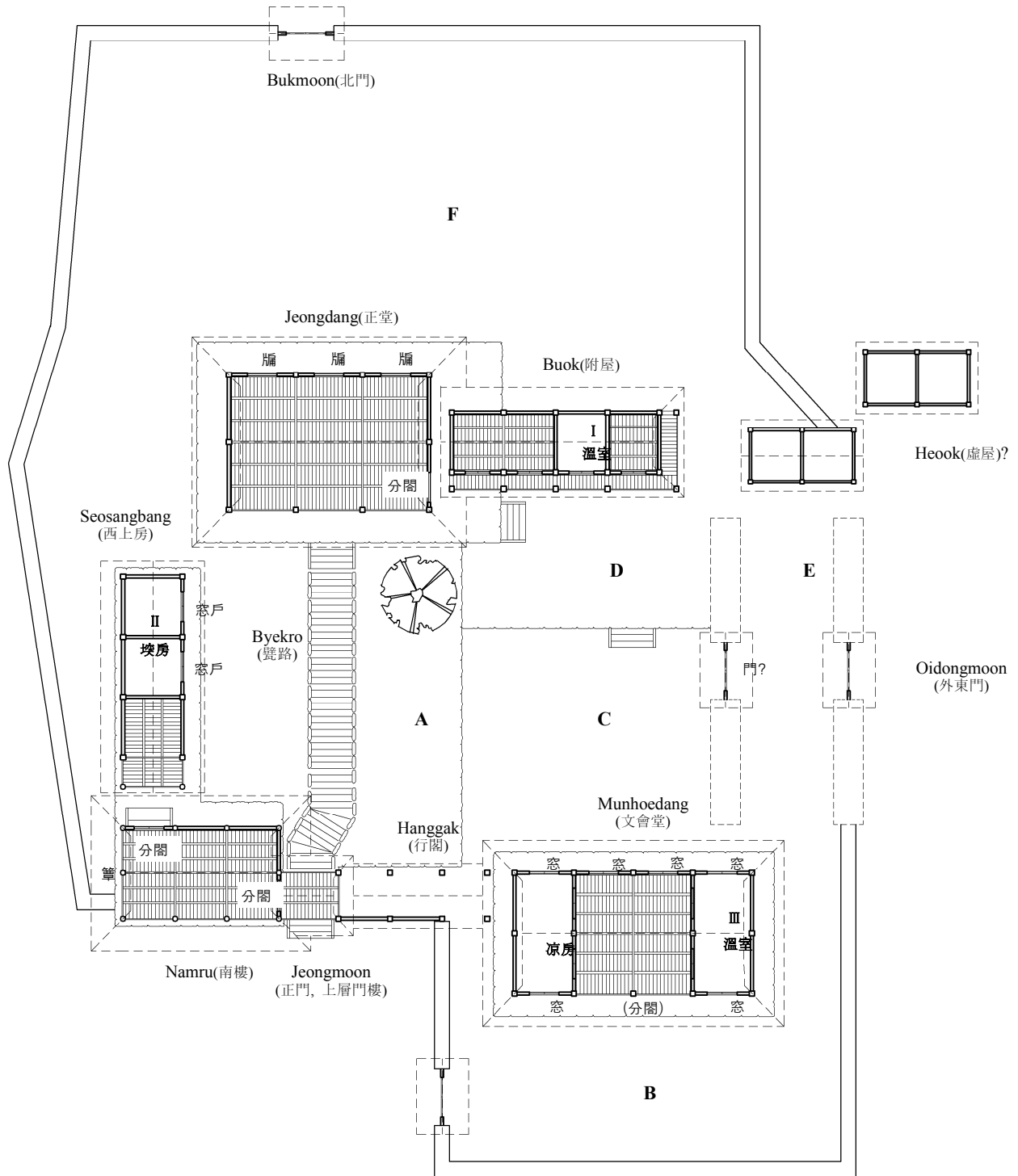
Figure 8. Reconstruction Drawing of DonghoDokseodang(東湖讀書堂) in late 16 th Century(Non scale) 39)
